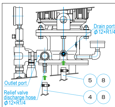
Pump side view from arrow A direction
